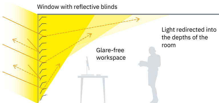
The upper section of the blinds directs the light into the depth of the room. The lower section enables glare-free light redirection to the ceiling.
